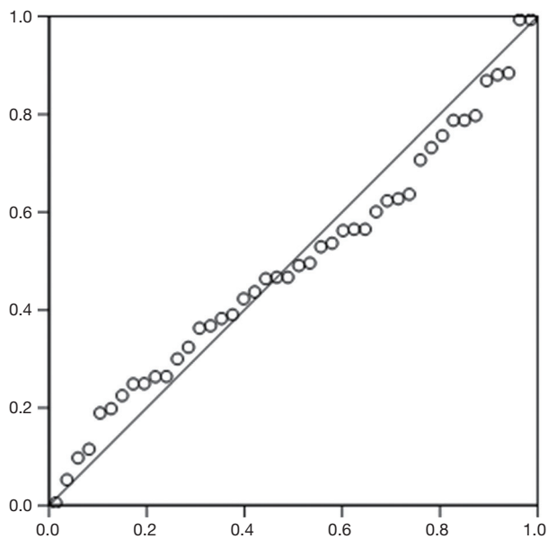
Figure 3 The normal P-P plot of regression standardized residuals (dependent variable: Y, independent variables for the cumulative probability, the abscissa is the observed cumulative feasibility and the ordinate is the expected cumulative feasibility).
