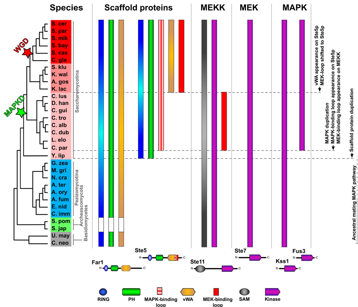
FIG 7 Architectural evolution of the mating MAPK signaling cascade during fungal evolution. Proteins are represented by their structural domains/motifs, which, if detected within a species, are marked in the table according to the color code indicated at the bottom. Major evolutionary steps are described on the right.
