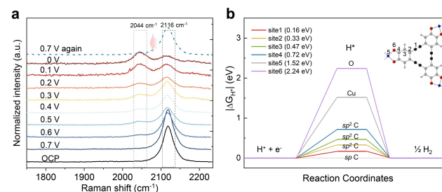
Figure 5. a) Potential-dependent Raman spectra of \text{Cu}_3\text{HHAEE}_2 in 0.1 M \text{Na}_2\text{SO}_4 under 594 nm laser excitation (QCP, open circuit potential). Operando resonance Raman spectra. b) Free-energy diagram for \text{H}_2 -evolution via a single-site reaction pathway: 1, 2, 3, 4, 5, 6 denote different active sites of \text{Cu}_3\text{HHAEE}_2 .
