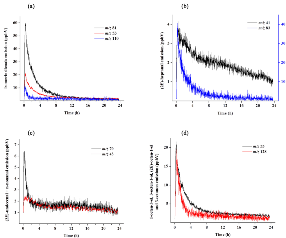
Figure 3. Time course of VOCs emission from rustyback fern ( A. ceterach ) fronds during the process of rehydration detected on-line by the PTR–MS method. Different colors indicate different ions corresponding to distinct volatiles: (a) Isomeric dienals, m/z 81 + m/z 53 + m/z 110; (b) (2E)-heptanal, m/z 83 + m/z 41; (c) (2E)-undecenal + n-nonanal, m/z 70 + m/z 43; (d) 1-octen-3-ol + 3-octen-1-ol + (2E)-octen-1-ol + 3-octanon, m/z 55 + m/z 128. Data shown represent mean sequence of plants from five independent experiments normalized to DW values.
