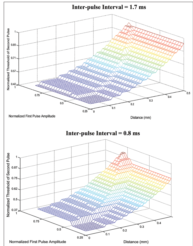
Figure 6: Characteristic of the second pulse threshold with respect to both electrode-to-fiber distance and the first pulse amplitude
