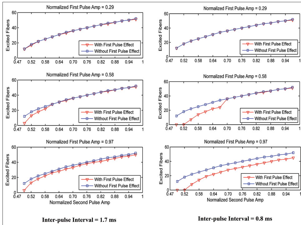
Figure 7: The number of excited fibers with respect to the second pulse amplitude. From top to bottom: the normalized amplitude of the first pulse is equal to 0.29, 0.58, and 0.97
