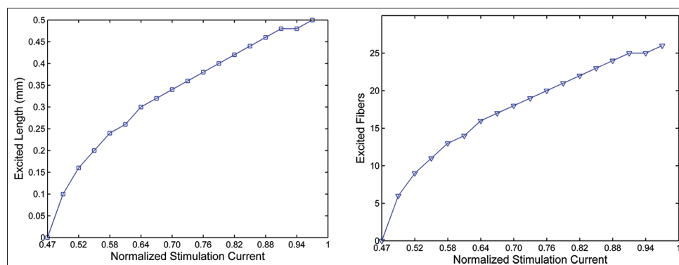
Figure 4: The length of the excited cochlear region and the number of excited fibers predicted by the Approximate Method
