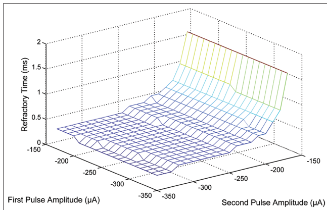
Figure 5: The refractory time changes of a nerve fiber's response to two sequential pulses
