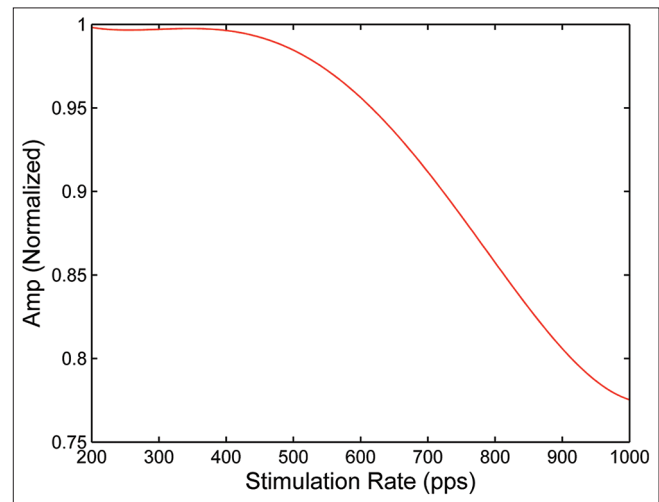
Figure 10: Normalized evoked compound action potential amplitudes averaged across pulses as a function of stimulation rate
