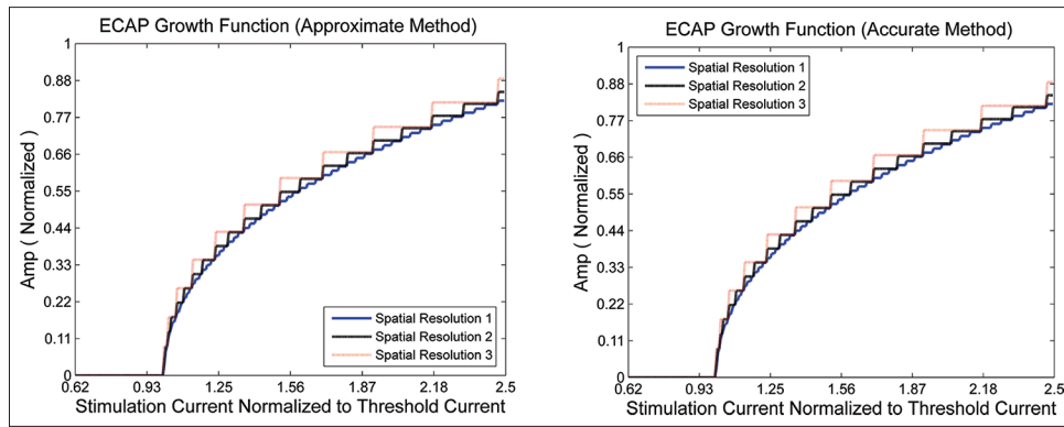
Figure 9: The normalized growth function obtained by the approximate and the accurate methods for different spatial resolutions and with the assumption of spatial resolution 1 > spatial resolution 2 > spatial resolution 3
