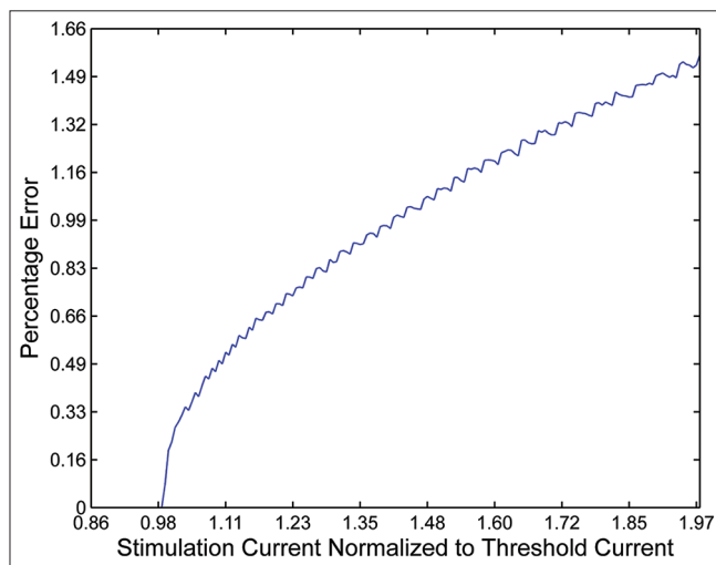
Figure 3: The simulation error of growth function resulted from the approximate method
