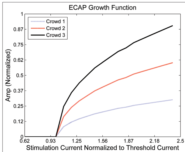
Figure 8: The normalized growth function with respect to different fiber density. It is assumed that Crowd represents the number of fibers and Crowd 3 > Crowd 2 > Crowd 1
