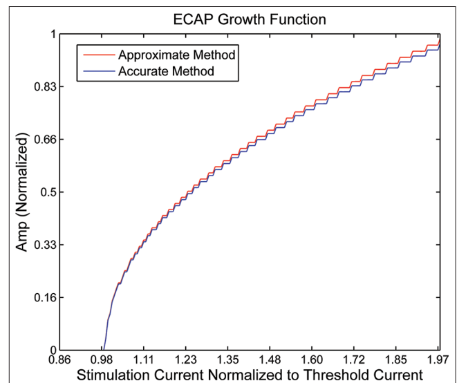
Figure 2: Comparing the growth functions acquired from approximate and accurate methods
