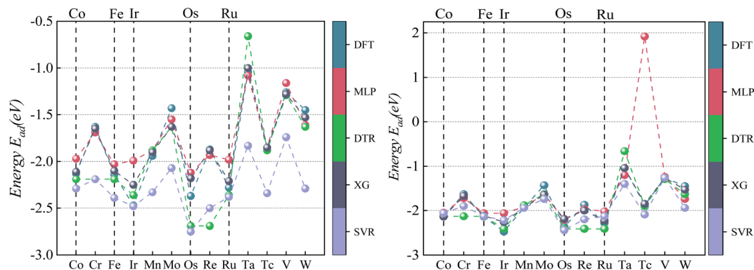
Fig. 8 Comparison of \text{CO}_2 E_{\text{ads}} between four ML predictions and DFT: prediction 1 (left); prediction 2 (right).
