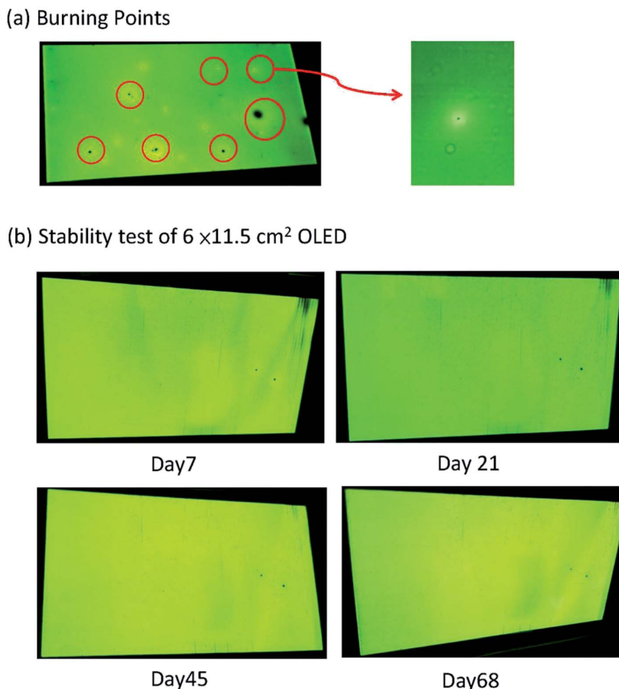
Fig. 19 (a) Burning points of OLED. (b) Stability test results of 6 \times 11.5 \text{ cm}^2 OLED with no burning point defects appearing after operating for over 1600 h (68 days).
