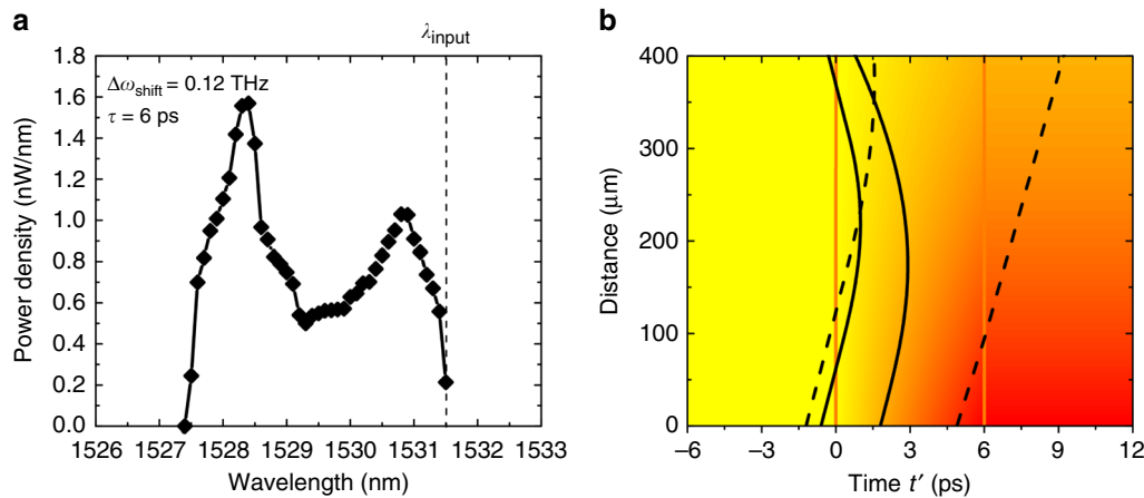
Fig. 5 Simulation of the FC front interaction with CW probe wave packets via ray tracing. a Wave packets average power spectrum for 6\ \mu\text{W} average power of the CW probe at 1531.5\ \text{nm} , rising time of the front of 6\ \text{ps} , and initial band shift \Delta\omega_{\text{shift}} of 0.12\ \text{THz} . Other parameters are listed in the Supplementary Note 6. b The trajectories of the probe wave packets with respect to the front velocity. The two vertical orange lines represent the extent of the index front with a rise time of 6\ \text{ps} , while the shading represents the refractive index front as it exponentially decays during propagation inside the waveguide. Solid black lines represent those wave packets that undergo complete transitions, while the dashed lines depict the wave packets which only undergo incomplete transitions
