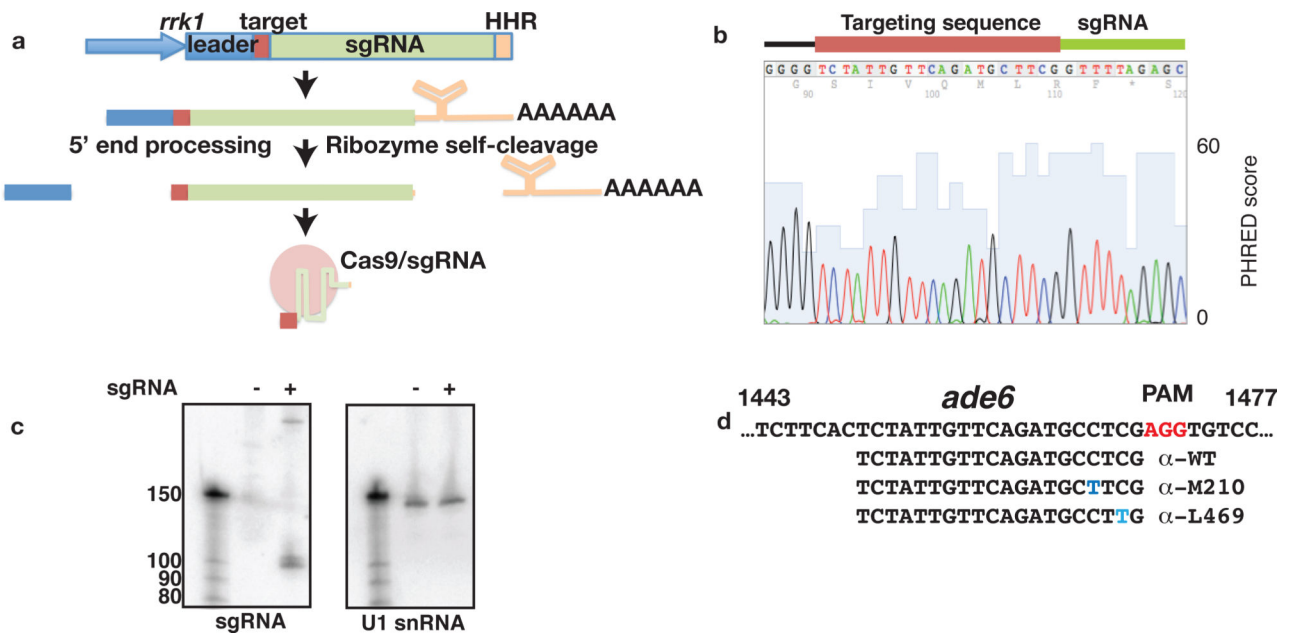
Figure 1. sgRNA expression system. (a) Schema of sgRNA expression construct and processing. HHR: Hammerhead Ribozyme. (b) 5' RACE sequence. Only 4bp of the oligodG attached to the 5' end, resulting from the method, are shown. (c) Northern analysis of Cas9 expressing, ade6 + strains with either no sgRNA vector or a sgRNA vector targeted against ade6-M210 . Marker sizes are shown to the left and hybridization probe below. (d) ade6 targeting sequences.
