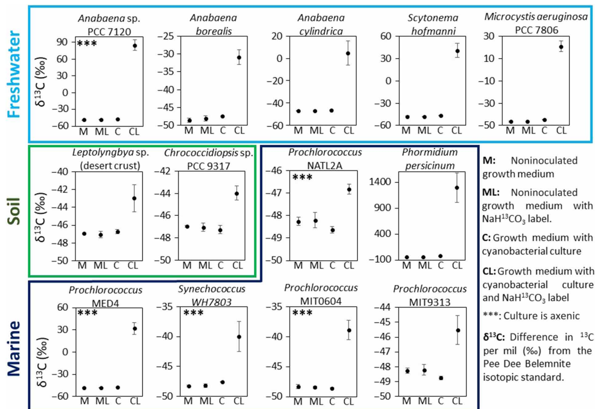
Fig. 1. \delta^{13}\text{C} - \text{CH}_4 values measured during incubation experiments of 13 different filamentous and unicellular freshwater, soil, and marine cyanobacterial cultures with and without \text{NaH}^{13}\text{CO}_3 supplementation. All cyanobacterial cultures produced \text{CH}_4 . Using \text{NaH}^{13}\text{CO}_3 as carbon source (CL) resulted in increasing stable \delta^{13}\text{C} - \text{CH}_4 values as compared to the starting condition. This establishes the direct link between carbon fixation and \text{CH}_4 production. The ^{13}\text{C} enrichment is not quantitative and thus not comparable between cultures. Error bars represent SD ( n = 4 ).
