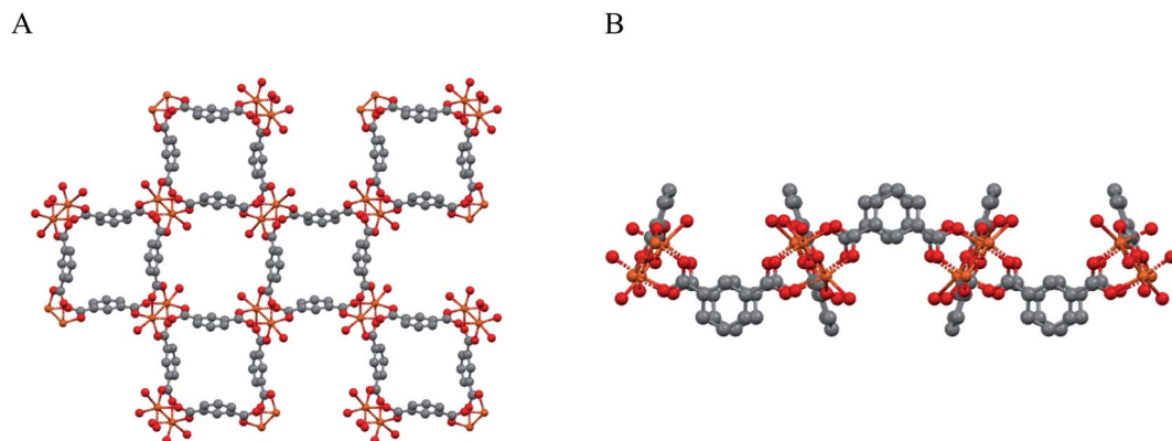
Fig. 3 Sketches of the weakly corrugated 2D layers in the crystal packing of \text{Cu}_2(\mu\text{-isophthalate})_4\text{D}_2 , present also in [\text{Cu}(\text{1,3-YBDC})] \cdot x\text{H}_2\text{O} . (A) View down [001]. (B) View down [100]. Note that, in [\text{Cu}(\text{1,3-YBDC})] \cdot x\text{H}_2\text{O} , the layers are not separated, but are interlinked by the long propargyl carbamate residues (in both a and b conformations) completing the \text{Cu}_2(\mu\text{-COO})_4 coordination sphere (the apical D atom) with a truly 3D connectivity.
