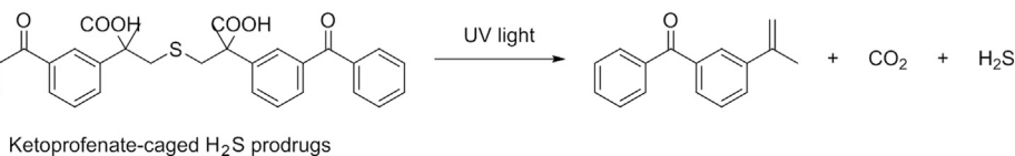
Scheme 7 H 2 S release from photo-induced H 2 S prodrugs.
