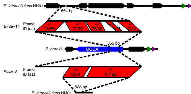
Figure 4 | GOGAT gene remnants in Richelia . The intergenic space between two R. intracellularis HH01 ORFs, including an annotated 120 bp hypothetical protein (in grey, RintHH_15420) compared with the gene encoding GOGAT in Raphidiopsis brookii D9 (in blue, CRD_00957) and the genomic context of each. The middle alignment represents the top BLAST hit of the R. intracellularis HH01 intergenic space (1561 bp) in the nr database (BLASTx, E -value = 3e^{-14} ). The green and purple genes encode a mannose-6-phosphate isomerase and a probable iron binding protein, respectively.
