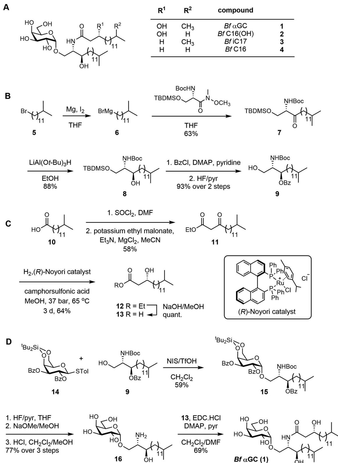
Fig. 1 Total synthesis of a representative B. fragilis α-galactosylceramide and acyl chain variants. (A) Structure of Bf αGC (αGalCer Bf -716 ) 1 , and analogues 2–4 . (B) Synthesis of the protected sphinganine 9 . (C) Synthesis of the b -hydroxy acid side-chain. (D) Assembly of Bf αGC. For synthesis of variants, see ESI.†
