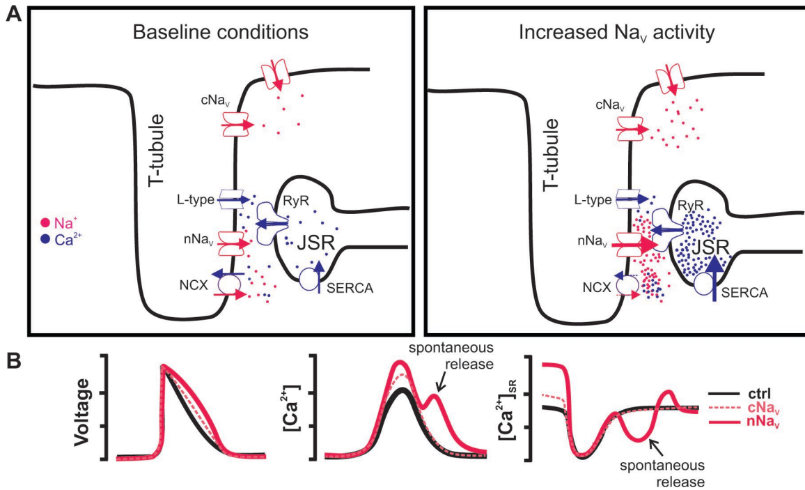
Figure 1. The proximity of \text{nNa}_v s to the excitation–contraction coupling machinery can be proarrhythmic. (A) Inferred locations of proteins important in excitation–contraction coupling are shown under control conditions (left) and after augmentation of flux through \text{Na}_v s (right). Compared with \text{cNa}_v s, \text{nNa}_v s appear to be located closer to the excitation–contraction coupling machinery, including LTCCs and \text{NCX} in the T-tubule membrane and \text{RyR} s and \text{SERCA} in the local SR membrane. An increase in \text{Na}^+ influx through \text{nNa}_v s will lead to increased local [\text{Na}^+] (red dots), reduced \text{Ca}^{2+} removal via \text{NCX} , and increased SR [\text{Ca}^{2+}] (blue dots). (B) Hypothetical action potentials (left), intracellular [\text{Ca}^{2+}] (middle), and SR [\text{Ca}^{2+}] (right) under control conditions (solid black lines), after augmentation of \text{cNa}_v s (dashed red lines), and after augmentation of \text{nNa}_v s (solid red lines). Increased flux through either \text{cNa}_v s or \text{nNa}_v s will prolong the AP and increase SR [\text{Ca}^{2+}] load. When this occurs through \text{nNa}_v s, however, the local signaling means that the increase in SR [\text{Ca}^{2+}] will be greater, increasing the risk of spontaneous, arrhythmogenic \text{Ca}^{2+} release.
