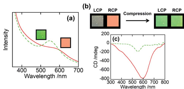
Fig. 5 (a) Visual appearances and UV-Vis spectra, (b) visual appearances through circular polarizers, and (c) CD spectra for 76 wt% PHPC/PACMO film before (—) and after (---) compression at 30 °C. The applied compressive strain and stress were 0.10 and ~5000 MPa, respectively.
