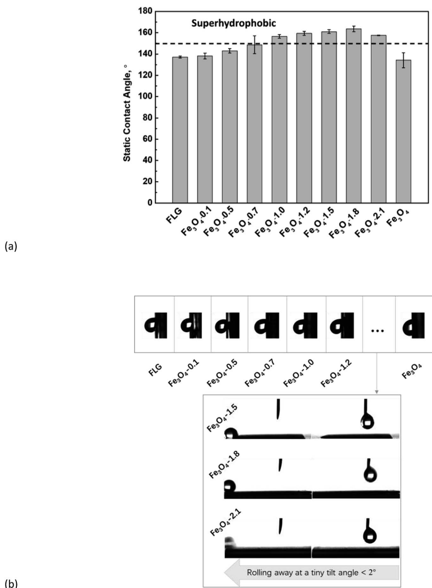
Fig. 4 (a) Variation of water static contact angles on bare \text{Fe}_3\text{O}_4 , FLG, and \text{Fe}_3\text{O}_4/\text{FLG} hybrid coatings \text{Fe}_3\text{O}_4 -0.1, \text{Fe}_3\text{O}_4 -0.5, \text{Fe}_3\text{O}_4 -0.7, \text{Fe}_3\text{O}_4 -1.0, \text{Fe}_3\text{O}_4 -1.2, \text{Fe}_3\text{O}_4 -1.5, \text{Fe}_3\text{O}_4 -1.8, \text{Fe}_3\text{O}_4 -2.1. (b) Sliding angle measurements: the adhesive performance is demonstrated by a water drop clinging to the vertical coatings wall, on bare FLG, \text{Fe}_3\text{O}_4 coatings, and \text{Fe}_3\text{O}_4/\text{FLG} hybrid coatings with 0.1, 0.5, 0.7, 1.0, 1.2 g \text{Fe}_3\text{O}_4 . Droplet quickly rolled off from \text{Fe}_3\text{O}_4/\text{FLG} hybrid coatings with 1.5, 1.8, and 2.1 g \text{Fe}_3\text{O}_4 at a tiny sliding angle < 2^\circ .
