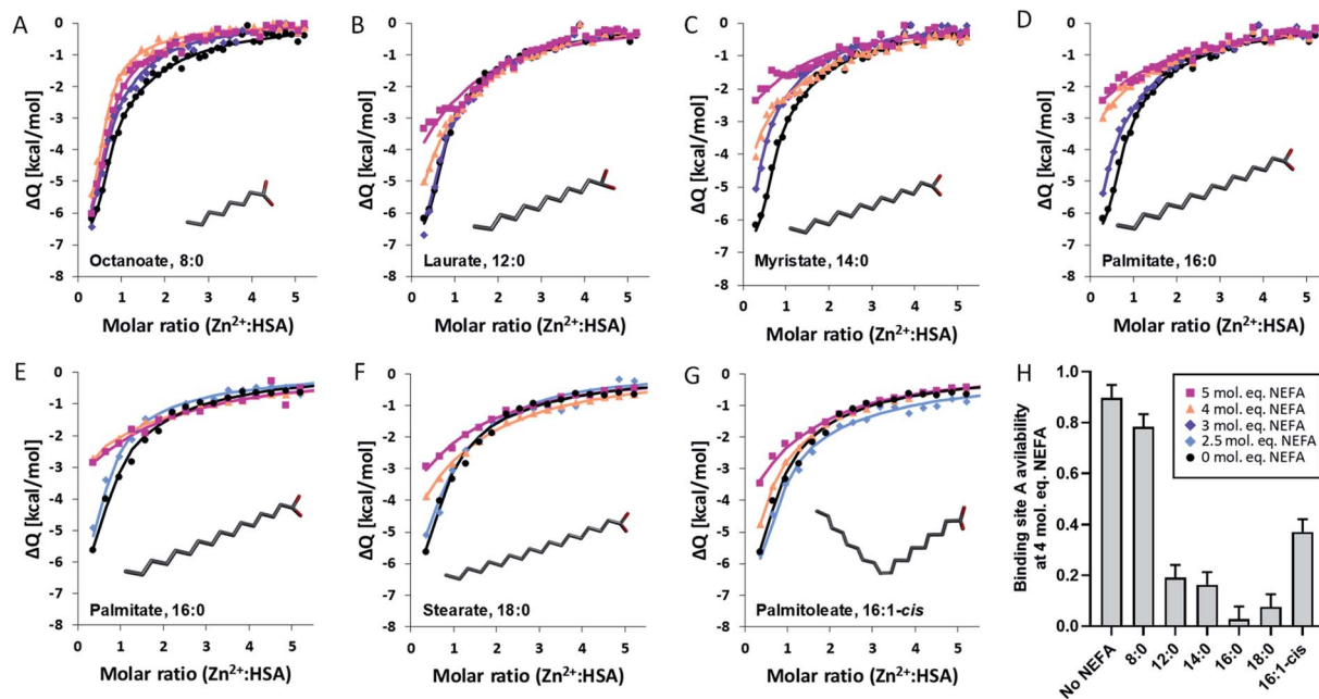
Fig. 2 Binding of Zn^{2+} to HSA in presence of different NEFAs. ITC experiments were conducted in a buffer containing 50 mM Tris, 140 mM NaCl, pH 7.4. A first set of experiments was performed with 1.5 mM ZnCl_2 titrated into 60 \mu M HSA, in the presence of either 0 (black), 2.5 (pale blue), 3 (dark blue), 4 (orange) or 5 (purple) mol. eq. of different NEFAs: (A) octanoate, (B) laurate, (C) myristate and (D) palmitate. The settings used were 25 ^{\circ} C, 39 injections (first injection was 0.4 \mu L, the remaining injections were 1 \mu L, initial delay 60 s and spacing 120 s). A second set of experiments was performed with 750 \mu M ZnCl_2 titrated into 25 \mu M HSA, in the presence of (E) palmitate, (F) stearate and (G) palmitoleate. For those ITC experiments, the settings were adjusted to 25 ^{\circ} C, 19 injections (first injection was 0.4 \mu L, the remaining injections were 2 \mu L, initial delay 60 s and spacing 120 s). Each fit corresponds to a two-sets-of-sites model. (H) Bar chart representing the availability of binding site A in the presence of 4 mol. eq. of various NEFAs (the values for palmitate measured with 25 and 50 \mu M HSA were averaged) and the average for all values obtained in the absence of NEFA (both at 50 \mu M and 25 \mu M HSA). The data are represented as mean \pm SD, with the SD obtained in the absence of NEFA used to estimate the other SD values. All NEFAs except octanoate perturbed Zn^{2+} -binding to the protein, with the effect increasing with the concentration of NEFAs.
