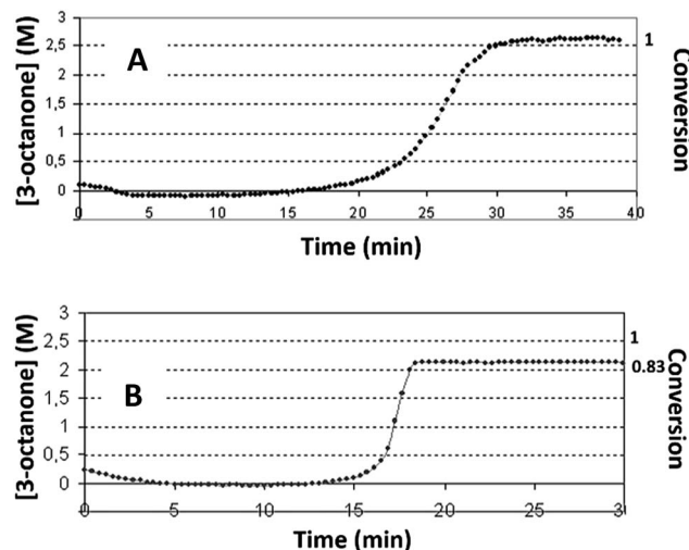
Fig. 1 The profiles of reaction (1) obtained with iso-propanol solvent under the following conditions: (A) – [Complex] 0 = 2.8 \times 10^{-4} (M), [S] 0 = 2.7 (M), conversion = 1.0 \pm 0.04 ; (B) – [complex] 0 = 1.48 \times 10^{-4} (M), [reactant 1] 0 = 2.7 (M), conversion = 0.83 \pm 0.05 .
