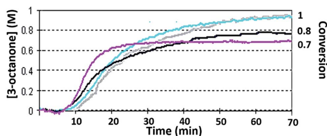
Fig. 8 Reaction (1) profile obtained under the following conditions: solvent – n -pentanol, TON = 3.91 \times 10^4 \pm 250 , [\text{reactant } 1]_0 = 0.99 (M), [\text{cat}]_0 = 2.5 \times 10^{-5} (M). Black – original conditions, TOF = 5.7 \times 10^2 \pm 50 (min -1 ), V_{\max} = 0.05 \pm 0.01 (M min -1 ), conversion = 0.7 \pm 0.05 . Purple – with fast stirring, TOF = 5.5 \times 10^2 \pm 50 (min -1 ), V_{\max} = 0.38 \pm 0.01 (M min -1 ), conversion = 0.81 \pm 0.05 . Blue – addition of [Aliquat] = 0.043 (M), TOF = 7.5 \times 10^2 \pm 50 (min -1 ), V_{\max} = 0.042 \pm 0.01 (M min -1 ), conversion = 1 \pm 0.05 . Grey – addition of [Aliquat] = 0.043 (M) and stirring, TOF = 7.2 \times 10^3 \pm 60 (min -1 ), V_{\max} = 0.038 \pm 0.01 (M min -1 ), conversion = 1 \pm 0.05 .
