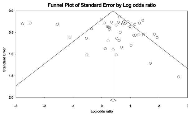
Fig. 2. Funnel plot of included studies.
