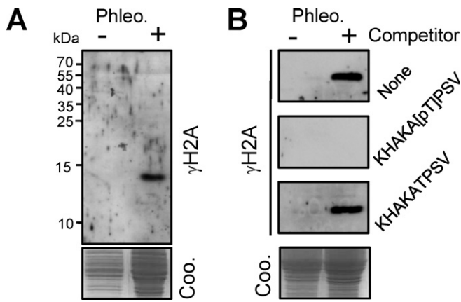
Fig. 2. Trypanosomal \gamma H2A is histone H2A phosphorylated at Thr 130 . (A) A western blot of whole T. brucei lysate before and after phleomycin (Phleo.) exposure shows that \gamma H2A levels increase following DNA damage. The coomassie (Coo.) panel shows loading. (B) The peptide competition assay demonstrates the specificity of the antibody. Other details are as for A.
