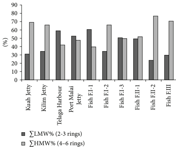
FIGURE 3: Relative percentages (%) of ΣLMW and ΣHMW in the sediment of different sampling stations.
