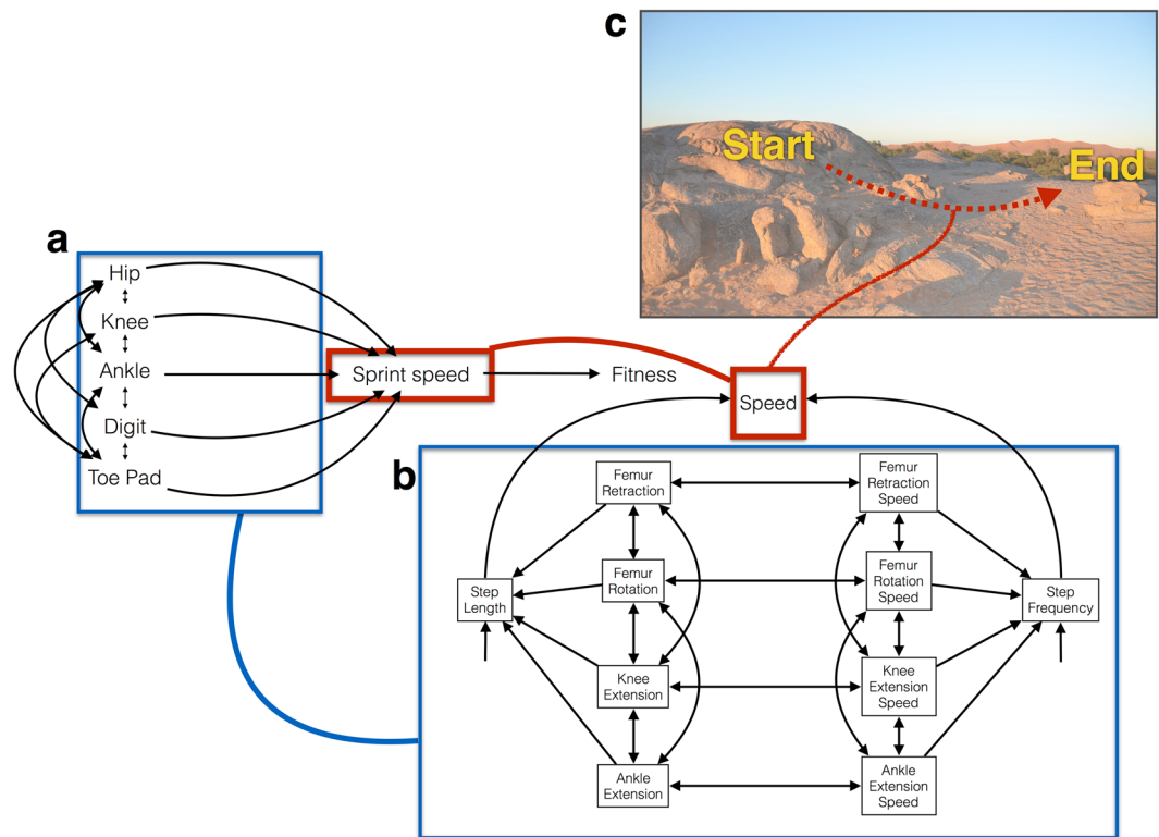
Figure 2. Conceptual model depicting the role of kinematics as the mechanistic linkage between animal morphology and performance in the context of physically challenging habitats. (a) We hypothesize that the kinematics studied in this experiment regulate how morphology determines performance in the Morphology → Performance → Fitness paradigm 7 . We focus on one type of performance, sprint speed. (b) A path model representing all possible kinematics that could have been measured in this study that lead to step length and step frequency, which in turn lead to speed. We focused on a subset of kinematics that theoretically determine performance on a level and an inclined surface. (c) Diagram composed of a photograph from the Gobabeb Research and Training Centre in Namibia and drawing depicting a typical escape path as previously described 31 .
