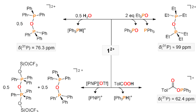
Scheme 3. Deoxygenation of \text{Et}_3\text{PO} , Water, p -Toluic Acid, and [\text{PNP}][\text{OTf}] by 1 2+ ; [\text{Al}^{\text{F}}] Anions Are Omitted for Clarity; All Reactions Were Conducted in o DFB at Ambient Temperature with Quantitative Conversion upon Mixing
