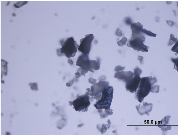
Figure 2- Micropol - irregular silicone carbide particles
