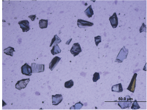
Figure 3- Opalustre - irregular silicone carbide particles
