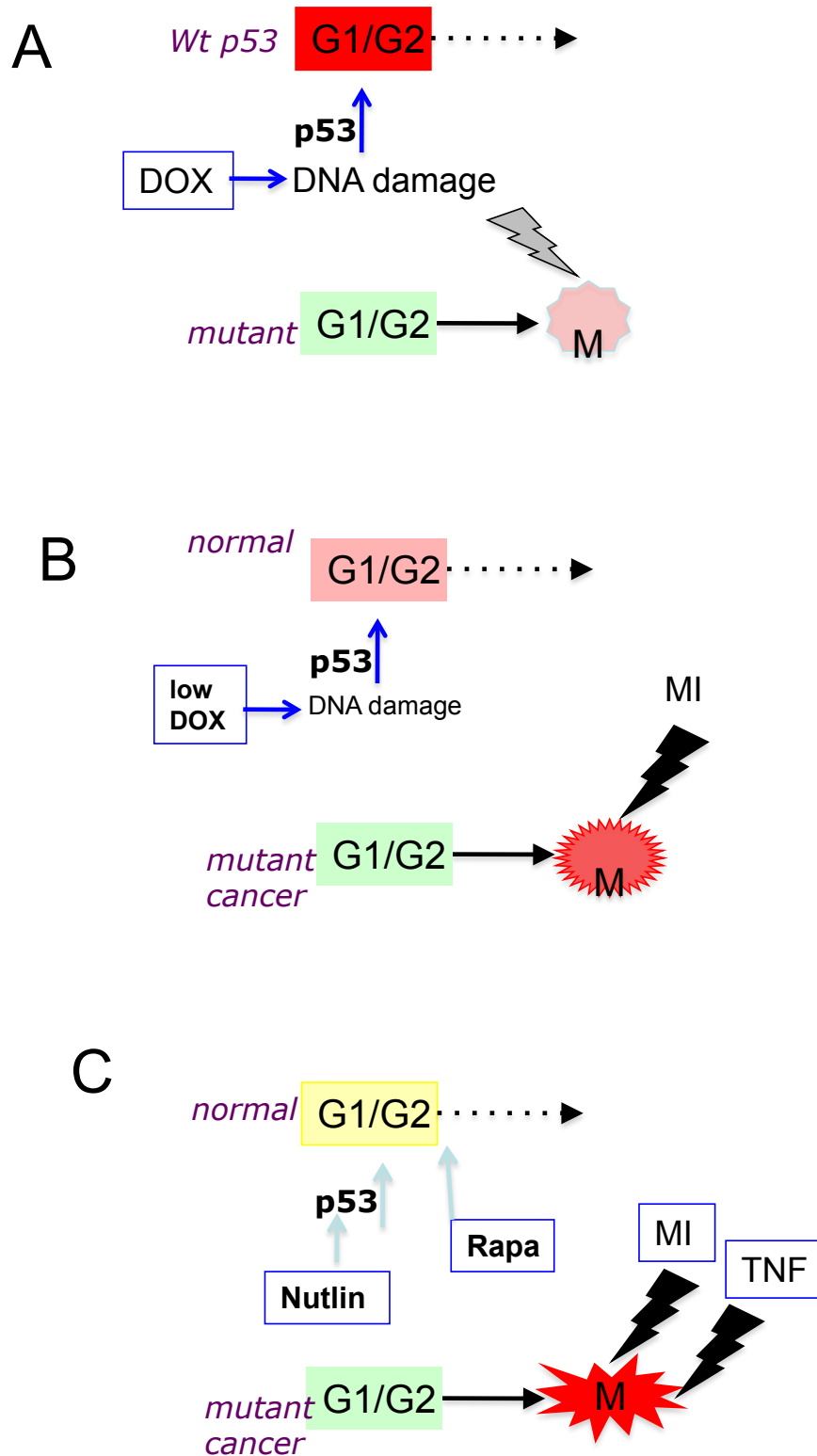
Figure 1: Protection of normal cells: From a single drug to ordered combinations. (A) Doxorubicin (Dox) causes G1/G2 arrest (red) in wt p53 cells, whereas cancer cells with mutant p53 enter mitosis (M) and undergo mitotic catastrophe. (B) Low doses of doxorubicin (low DOX) cause a more gentle G1/G2 arrest (orange) in normal cells, whereas cancer cells with mutant p53 enter mitosis (M) and are killed by MI (mitotic inhibitor such as Taxol). (C) Nutlin-3a plus rapamycin cause the gentlest G1/G2 arrest (yellow) in normal cells, whereas cancer cells with mutant p53 enter mitosis (M) and are killed by a highly apoptotic combination of MI plus TRAIL or TNF.
