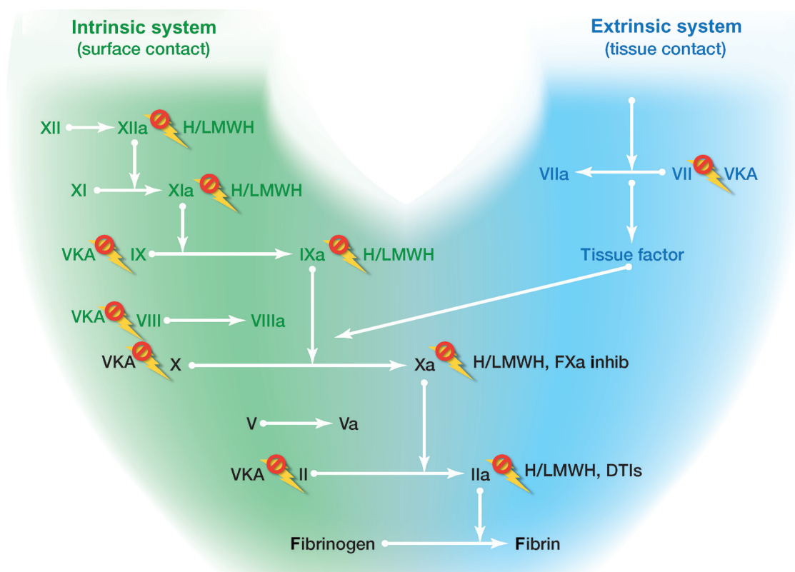
Figure 1 Coagulation cascade: targets for antithrombotic intervention.
