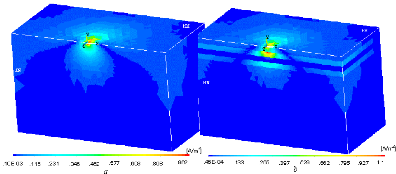
Figure 7 Distribution of the modulus of the current density vector in the homogeneous (a) and non-homogeneous (b) domains from a vertically positioned coil. Section and viewing angle – as in Fig. 4,5,6.
