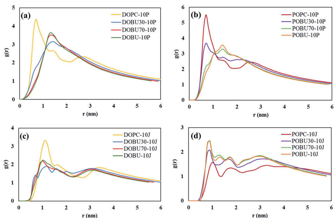
Fig. 7 Membrane–fullerene COM radial distribution functions for (a, b) pristine fullerenes, (c, d) Janus fullerenes at fullerene-to-lipid ratio of F/L = 10/512 .
