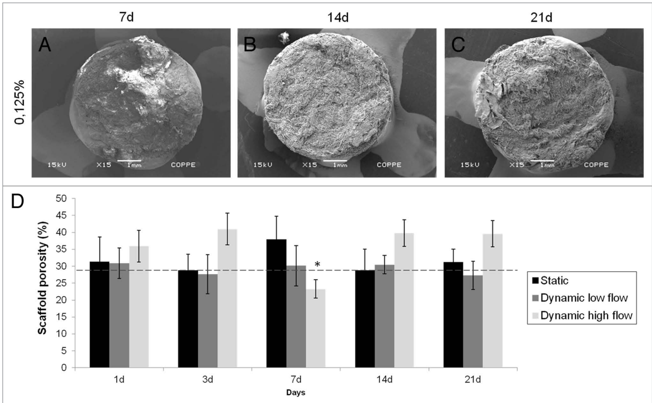
Figure 2. (A, B and C) SEM micrographs of scaffolds immersed under static culture condition up to 21 d and (D) total porosity of scaffolds maintained under different culture conditions up to 21 d. The dotted line indicates the initial porosity after 24 h under biological conditions. Error bars represent mean \pm SD with n = 4 . The symbol (*) indicates statistical significance within a timepoint ( p < 0.01 ).
