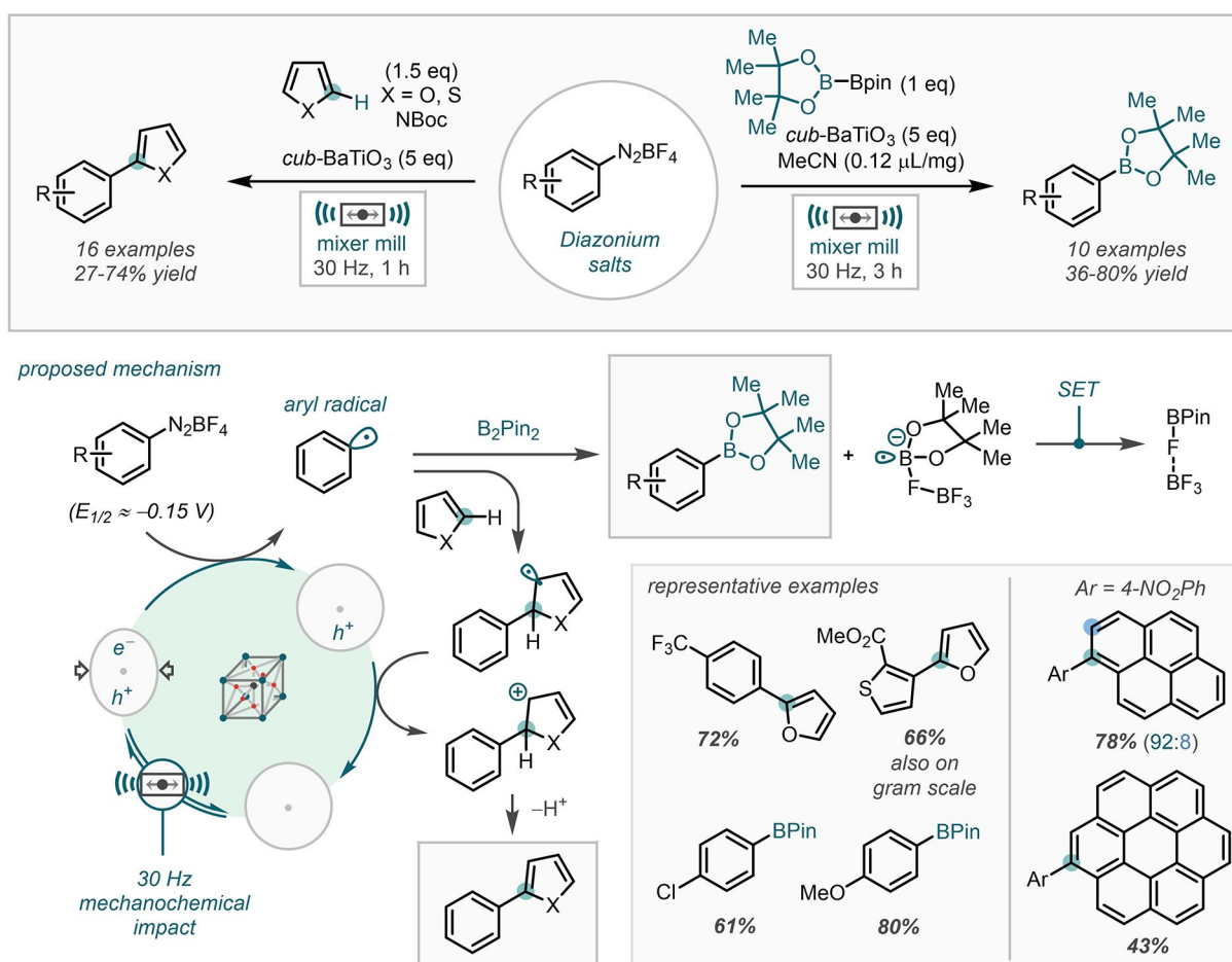
Scheme 2. Mechanoredox formation of aryl radicals using piezoelectric materials.
