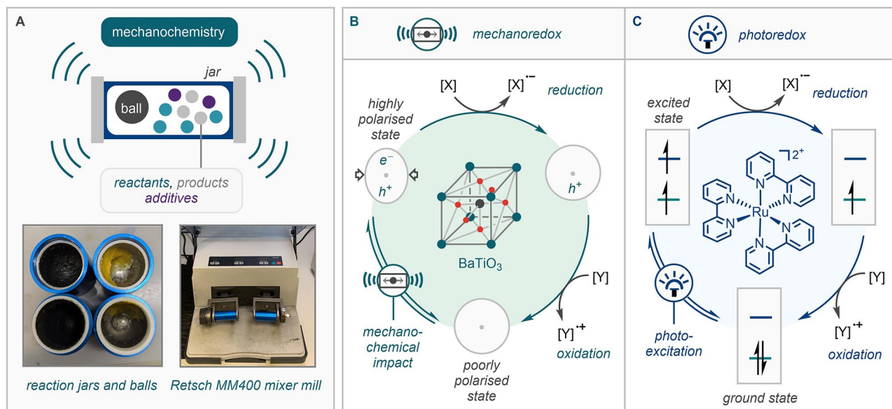
Scheme 1. Mechanochemistry and redox cycles in the context of photoredox and mechanoredox manifolds. Cubic BaTiO 3 shown as a representative piezoelectric material.
