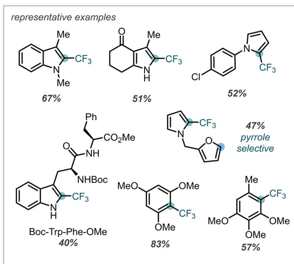
Scheme 4. Mechanochemical generation of trifluoromethyl radicals using piezoelectric materials.
