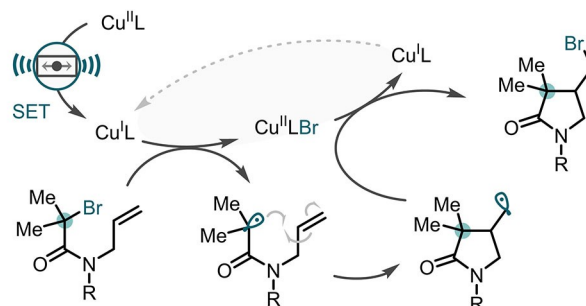
Scheme 3. Mechanoredox-triggered ATRC of alkene-tethered \alpha -bromoamides. TPMA = tris(2-pyridylmethyl)amine.
