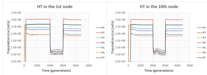
Figure 9 Population dynamics in the C-C community in the flow-through habitat. Chemotaxis is on (Additional file 3, Additional file 4).
