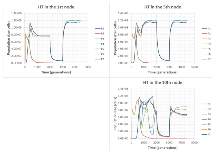
Figure 10 Population dynamics in the NC-NC community in the flow-through habitat. Chemotaxis on (Additional file 5, Additional file 6, Additional file 7).
