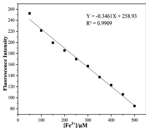
Fig. 3 Normalized response of fluorescence signal to \text{Fe}^{3+} in the range of 5 \times 10^{-5} to 5 \times 10^{-4} M.
