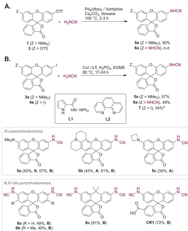
Fig. 2 Synthesis of N -cyano- and N,N' -dicyanorhodamine fluorophores under Buchwald–Hartwig (A) and Ullmann (B) reaction conditions. a Ligand L2 was used instead of L1 ; EGME – ethylene glycol monomethyl ether.
