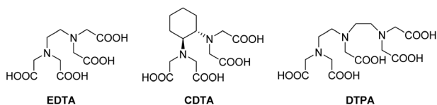
Scheme 1 Ligands discussed in the present work.
