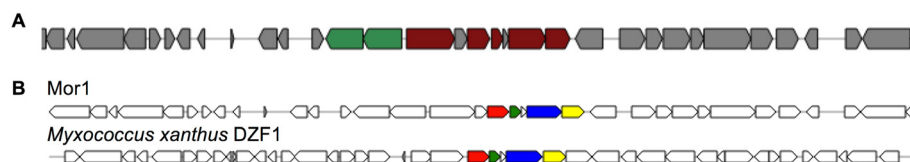
Fig. 1 Schematic of the polyketide synthase (PKS) type III pathway discovered within the Mor1 genome using antiSMASH [41]. a The entire Mor1 type III PKS gene cluster with maroon genes corresponding to biosynthetic genes, green genes corresponding to regulatory genes, and grey genes corresponding to other uncharacterized genes. This locus is located between nucleotides 1238773 – 1279822 of the genome. b The comparison of the Mor1 gene cluster with homologous areas within the alkyresorcylic acid pathway gene cluster in the genome of Myxococcus xanthus DZF1. The red arrow corresponds to a stilbene synthase gene with 58 % identity and 99 % coverage; the green arrow corresponds to a methyltransferase gene with 54 % identity and 85 % coverage; the blue arrow corresponds to an AMP-dependent synthetase with 54 % identity and 96 % coverage; the yellow arrow corresponds to a monooxygenase gene with 47 % identity and 69 % coverage. Images generated by antiSMASH [31]
