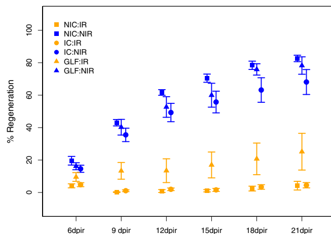
Fig. 2. Regrowth of caudal fin after dissection to test for somatic regeneration in males of all three treatments (GLF, IC, and NIC) with (IR) and without (NIR) irradiation measured from 6 to 21 dpi. Values displayed represent mean \pm SE.
