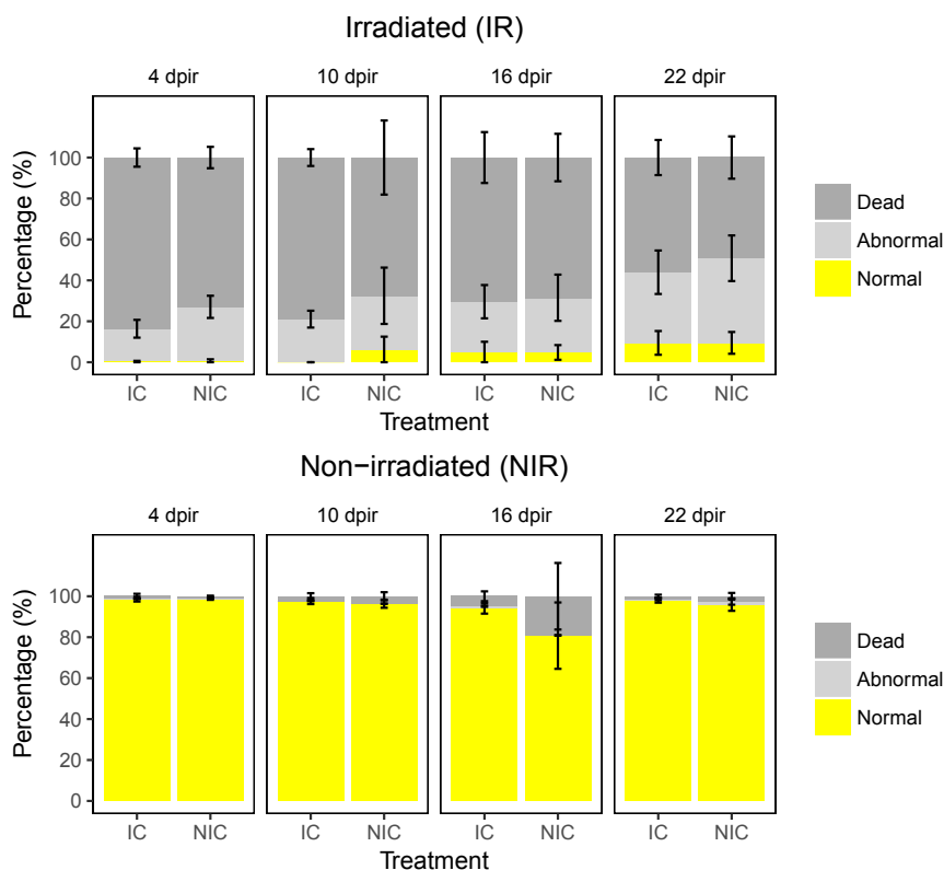
Fig. 1. Percentage of normal, abnormal, and dead embryos in the clutches laid by males in two different treatments of germline-carrying fish (IC and NIC) and subtreatments (IR, NIR) from 4 to 22 dpi. (Upper) Results for irradiated fish with a clear detrimental effect of irradiation on embryo survival and development. (Lower) Males of both treatments bred at the same time points without irradiation. Values displayed represent mean \pm SE. The amount of normal embryos differed significantly between treatments (irradiation: \chi^2_1 = 525.285 , P < 0.001 ; treatment: \chi^2_1 = 73.209 , P < 0.001 ; irradiation*dpi: \chi^2_3 = 26.407 , P < 0.001 ; see SI Appendix, Table S4 for full model).
