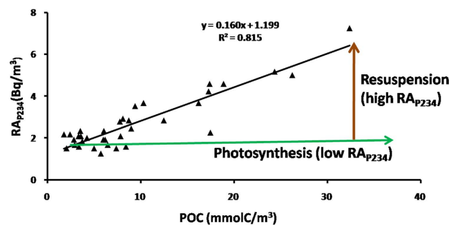
Figure 3. RA_{p234} versus POC in the western Arctic Ocean. The photosynthesis indicated by green arrow can elevate POC but lower RA_{p234} . Resuspension is represented by brown arrow and characterized by high RA_{p234} .
