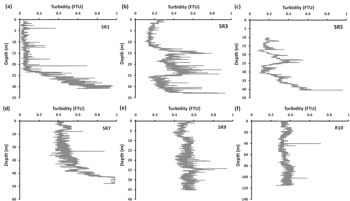
Figure 2. Seawater turbidity at stations SR1 (a), SR3 (b), SR5 (c), SR7 (d), SR9 (e), R10 (f).
