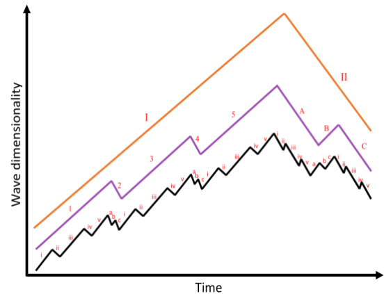
Figure 1. Elliott waves of smallest dimension (sub-waves; black) are shown along with the waves of higher dimensions (purple and orange). i, iii, v are impulses of the smallest dimension; 1, 3, 5 are impulses of next higher dimension; I is the impulse of next higher dimension. Similarly, ii and iv are correctives of the smallest dimension, 2 and 4 are correctives of the next higher dimension, and II is the corrective of next higher dimension. Impulses (e.g. I) are made up of 5 waves of lesser dimension (i.e. 1, 2, 3, 4, 5), while correctives (e.g. II) are made up of 3 waves of lesser dimension (i.e. A, B, C).
