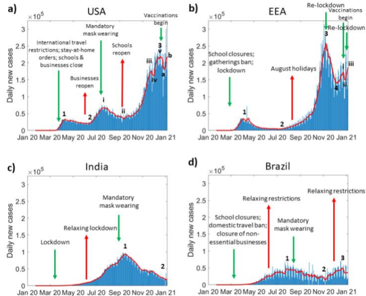
Figure 2. Daily new case timeline of COVID-19 in a) USA, b) European Economic Area (EEA), c) India, and d) Brazil, as of 1/5/2021. Red line represents seven-day moving average of the cases. Impulses 1, 3, 5, (or, i, iii, v) and correctives 2 and 4 (or, ii and iv) are shown wherever they are visible. Green and red arrows indicate the major restrictive and permissive events, respectively. Data source: https://github.com/owid/covid-19-data/blob/master/public/data/jhu/new_cases.csv
