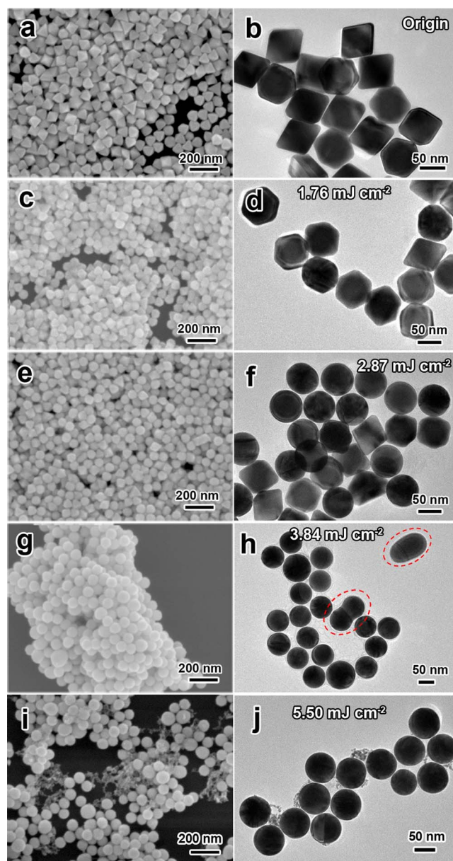
Figure 5 | SEM and TEM images of Au NPs obtained by laser irradiation ( \lambda = 532 nm, 20 Hz) at various laser fluences for 240 s. (a, b) original octahedral nanoparticles, (c, d) 1.76 , (e, f) 2.87 , (g, h) 3.84 and (i, j) 5.50 mJ cm ^{-2} .
