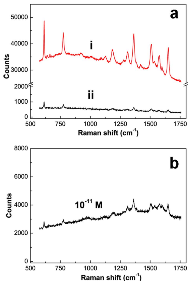
Figure 4 | SERS spectra of R6G molecules on different substrates. (a) after immersion in 10^{-6} mol L ^{-1} R6G solution for 30 min (Integral time: 1 s). Curves i: Au spherical nanoparticles array, Curve ii: a normal Au film (about 80 nm in thickness) prepared by sputtering deposition. (b) Raman spectra of R6G molecules on Au nanoparticle array after immersion in 10^{-11} mol L ^{-1} R6G solution. Note: the laser powers operated in (a) and (b) are 1 and 5 mW respectively.
