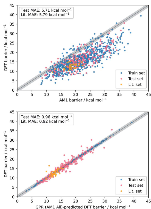
Fig. 3 Scatter plots showing the accuracy of DFT barrier prediction using only the AM1 barrier (top) compared to ML with GPR (AM1 All) (bottom), both with respect to the identity line (grey bands correspond to \pm 1 kcal mol -1 ).
