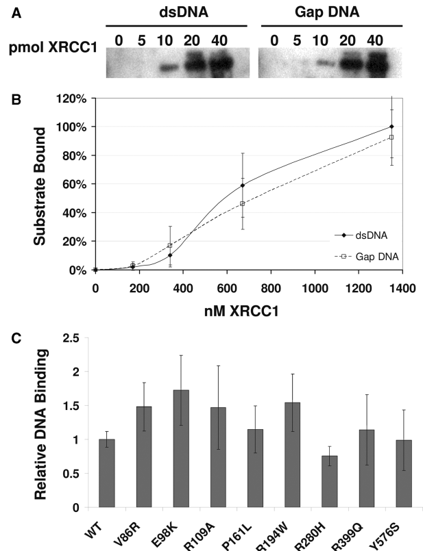
Figure 4. Binding of XRCC1 to DNA. (A) Representative WB blot. Indicated substrates (10 pmol) were captured on streptavidin beads and incubated with XRCC1 (5, 10, 20 or 40 pmol), and bound protein was pulled down and detected by WB. (B) Graph displaying full-length XRCC1 binding to unmodified duplex or single nucleotide gapped DNA substrates. Shown is the average and standard deviation of three independent experimental runs. (C) DNA-binding activities of the XRCC1 variants. Shown is a graph of the binding to Gap DNA of various XRCC1 mutant proteins compared to WT. Standard deviation of the values for the WT XRCC1 binding reactions is shown as well.
