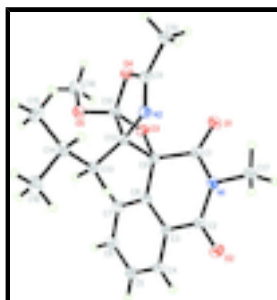
Fig. 1. The molecular structure of the title compound showing 50% probability displacement ellipsoids for non-H atoms.
