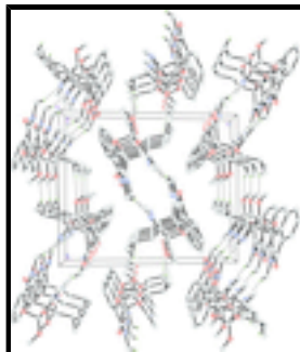
Fig. 2. Part of the crystal structure of the title compound, viewed along the a axis. H atoms not involved in hydrogen bonds (dashed lines) have been omitted for clarity.
