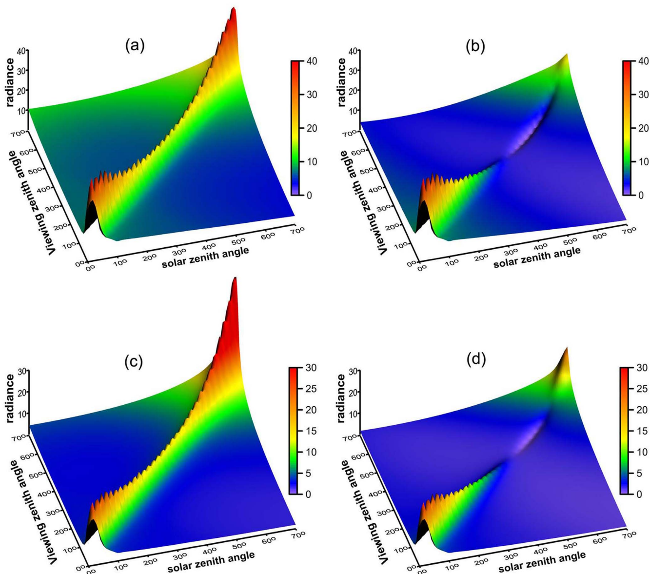
Figure 1 | The upward total radiance and PPR at the TOA simulated by PCOART. The radiances were observed in the specular plane corresponding to the solar incident direction with units of \text{mW}/(\text{cm}^2 \cdot \mu\text{m} \cdot \text{sr}) . The solar zenith angles were taken from 0^\circ to 70^\circ with a step of 1^\circ . It should be noted that the discrete peaks (sun glint) were caused by the discrete solar zenith angles with a step of 1^\circ , and the actual sun glint should be a continuous curve. (a) The total radiance at 443 nm, (b) PPR at 443 nm, (c) total radiance at 670 nm, (d) PPR at 670 nm.
