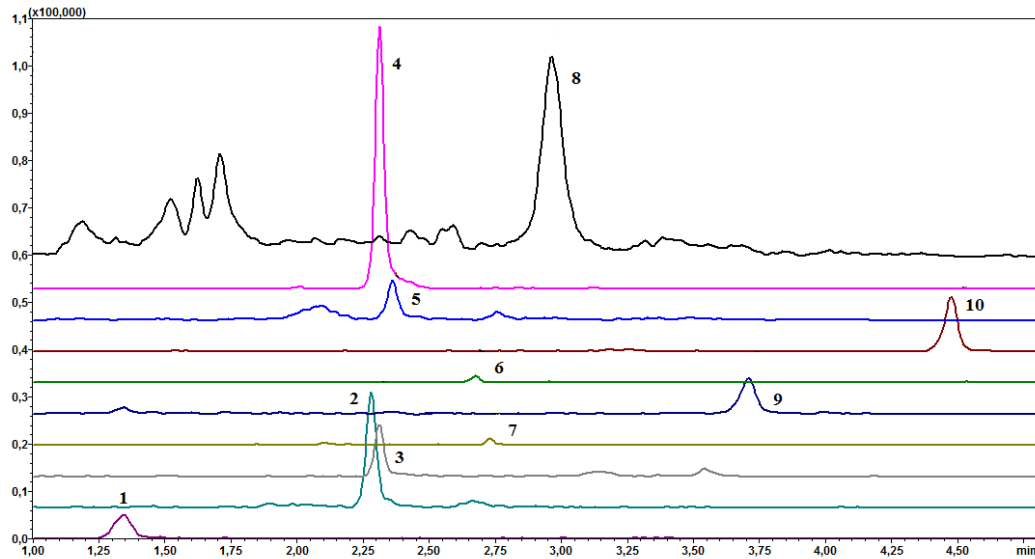
Fig. 1. Chromatograms of feed sample fortified with 10 dyes at 10 \mu\text{g}/\text{kg} and corresponding retention times (RT, min): 1. Sudan Orange G (1.343), 2. Sudan Red G (2.280), 3. Toluidine Red (2.311), 4. Citrus Red (2.312), 5. Sudan I (2.362), 6. Sudan IV (2.676), 7. Para Red (2.731), 8. Sudan II (2.963), 9. Sudan III (3.709), 10. Sudan Red 7B (4.476)
