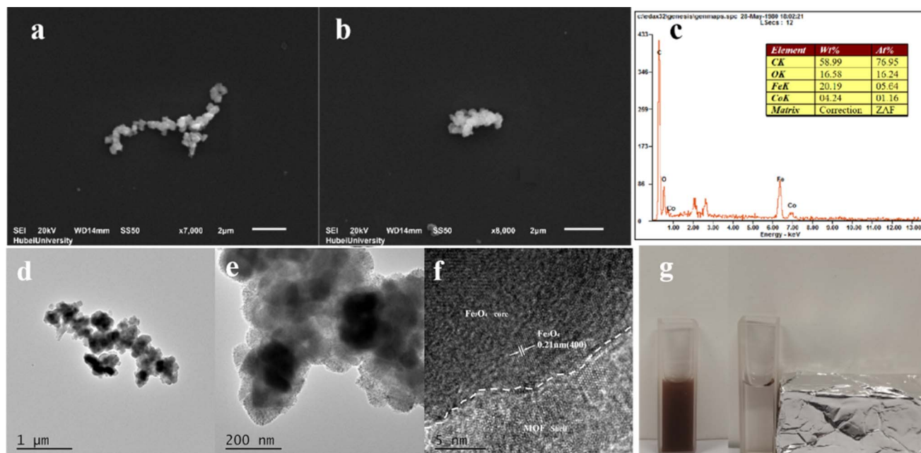
Fig. 2 SEM images of \text{Fe}_3\text{O}_4@MIL-101(\text{Fe, Co}) (a and b); the EDX spectrum of \text{Fe}_3\text{O}_4@MIL-101(\text{Fe, Co}) (c) HRTEM image of \text{Fe}_3\text{O}_4@MIL-101(\text{Fe, Co}) (d–f); changes of \text{Fe}_3\text{O}_4@MIL-101(\text{Fe, Co}) before and after magnetic field application (g).
