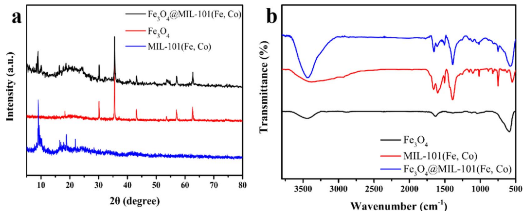
Fig. 1 (a) XRD of \text{Fe}_3\text{O}_4@MIL-101(\text{Fe, Co}) , MIL-101(\text{Fe, Co}) and \text{Fe}_3\text{O}_4 ; (b) FT-IR of \text{Fe}_3\text{O}_4@MIL-101(\text{Fe, Co}) , MIL-101(\text{Fe, Co}) and \text{Fe}_3\text{O}_4 .
