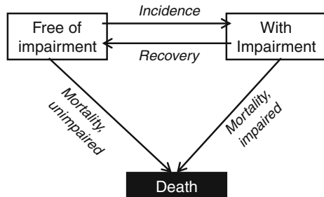
Fig. 1 Structure of a multi state life table model with two health states. The transitions are age dependent and conditioned by risk status
