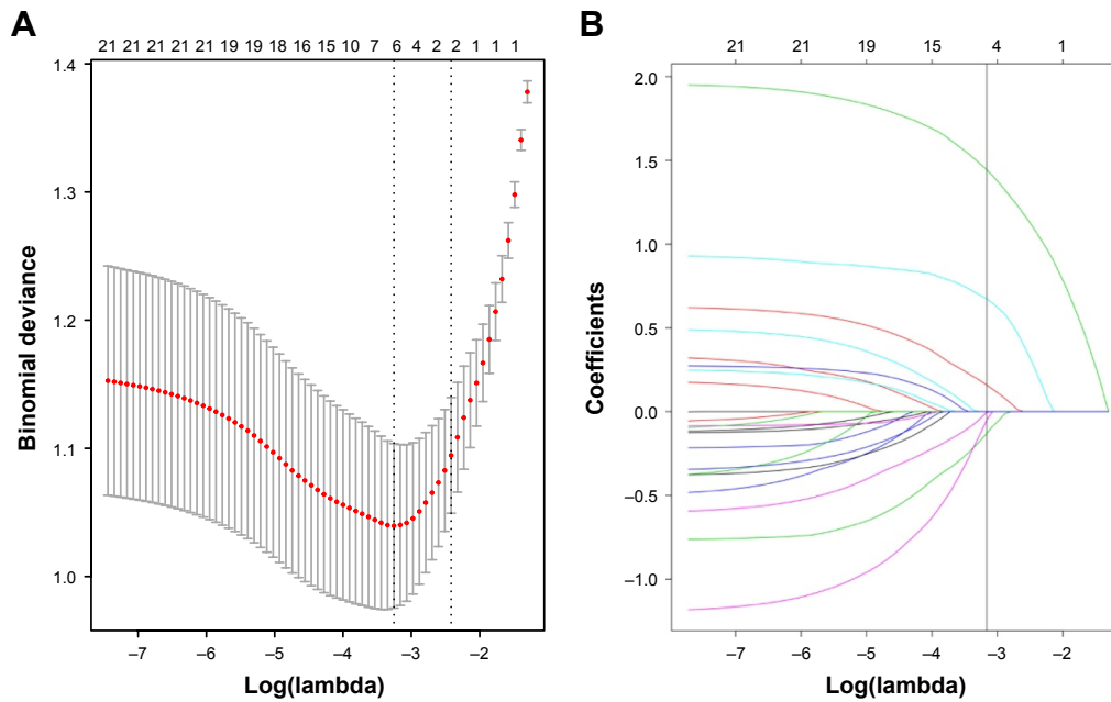
Figure 1 Demographic and clinical feature selection using the LASSO binary logistic regression model. Notes: (A) Optimal parameter (lambda) selection in the LASSO model used fivefold cross-validation via minimum criteria. 17,24 The partial likelihood deviance (binomial deviance) curve was plotted versus log(lambda). Dotted vertical lines were drawn at the optimal values by using the minimum criteria and the 1-SE of the minimum criteria (the 1-SE criteria). (B) LASSO coefficient profiles of the 22 features. A coefficient profile plot was produced against the log(lambda) sequence. Vertical line was drawn at the value selected using fivefold cross-validation, where optimal lambda resulted in five features with nonzero coefficients. Abbreviations: LASSO, least absolute shrinkage and selection operator; SE, standard error.
