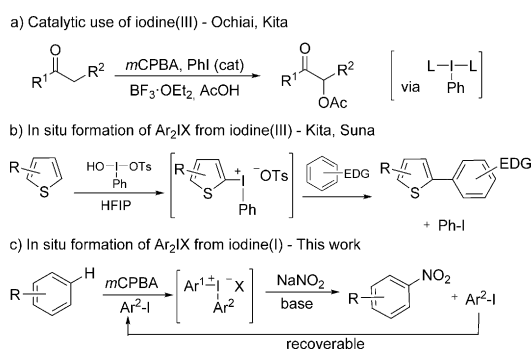
Scheme 1. In situ formation of iodine(III) reagents. EDG = electron-donating group, HFIP = 1,1,1,3,3,3-hexafluoro-2-propanol, mCPBA = m-chloroperbenzoic acid, Ts = 4-toluenesulfonyl.
