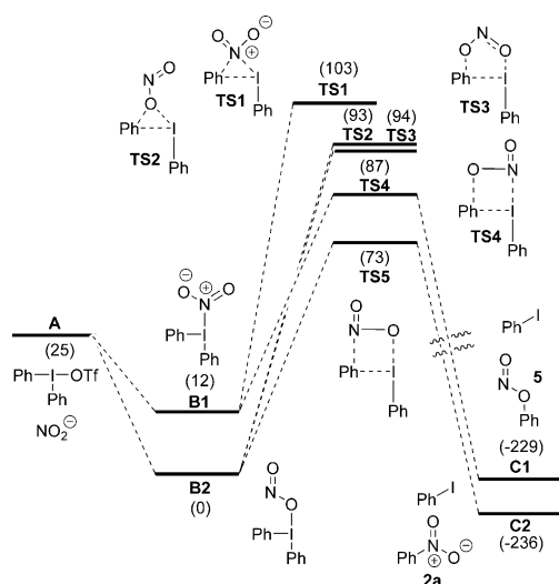
Figure 1. DFT calculated potential energy surfaces for the reaction between 1a (OTf) and nitrite. Energies are measured in \text{kJ mol}^{-1} . ^{-}\text{OTf} omitted for clarity in B1 and B2 , TS1 – TS5 , and C1 and C2 .
