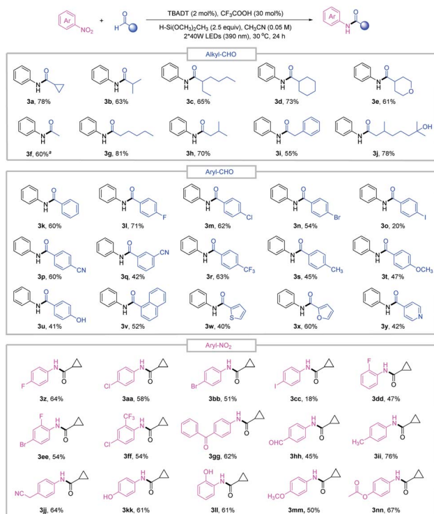
Fig. 2 Substrate scope of reductive amidation. Standard conditions: nitroarene 1 (0.1 mmol), aldehyde 2 (3 equiv.), TBADT (2 mol%), CF 3 -COOH (30 mol%), H-Si(OCH 3 ) 2 CH 3 (2.5 equiv.), CH 3 CN (0.05 M), purple LEDs (390 nm), 30 °C, 24 h. a The amount of aldehyde was 20 equiv.
